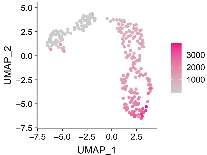
mouse_gene_count
