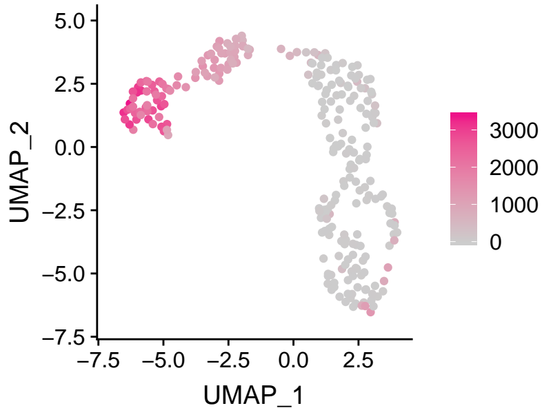
huamn_gene_count
